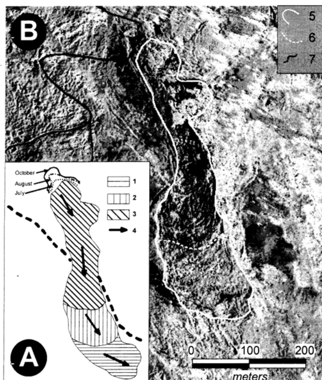
Fig.3. (A) SE2 Horizontal displacements from June 23, 1995 to October 14, 1995. Displacements rates (m/month): 1) 0.02 \pm 0.2 , 2) 0.4 \pm 10 and 3) 10 \pm 20 ; 4) main displacement direction. (B) Normalised difference ratios of SW and LW infra-red morning data. 5) SE2 landslide body; 6) separation line between different tone and texture areas; 7) main roads.
