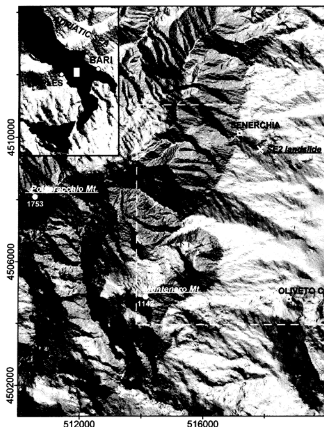
Fig.1. Twenty-meter resolution digital terrain model of the area represented as "real-time sun-shaded" image. The broken line is the Fig.3 boundary.
